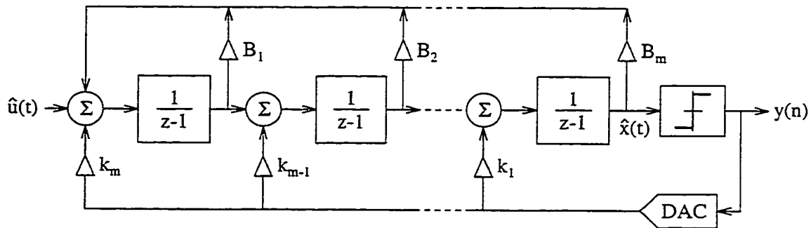
Figure 2.6: General m th-order low pass \Delta\Sigma M structure.
