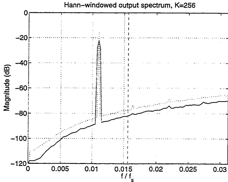
Figure 2.12: Hann-windowed averaged periodogram near dc.
