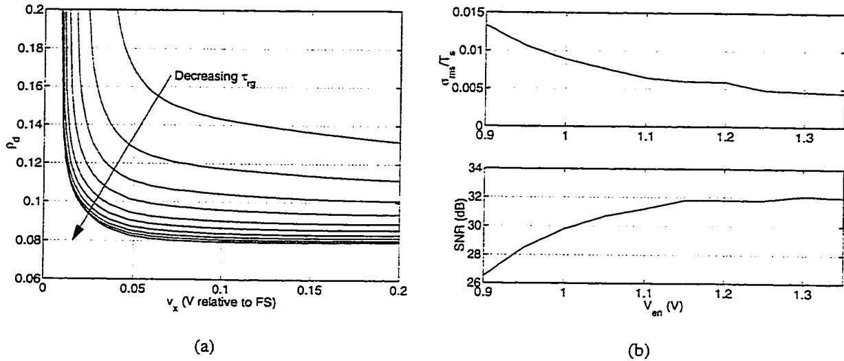
Figure 6.18: (a) Quantizer metastability curves and (b) modulator performance as a function of \tau_{rg} .
