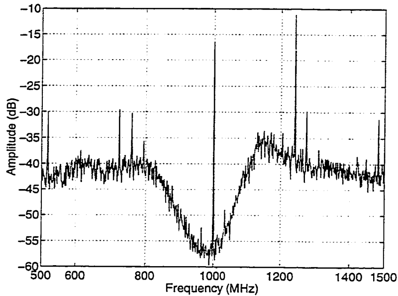
Figure 7.40: Output spectrum of captured bit stream.
