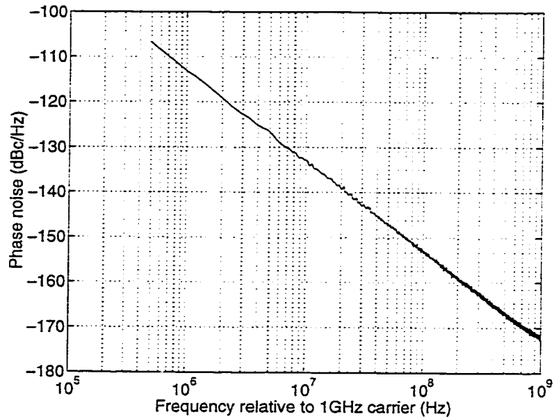
Figure 5.8: Phase noise plot for accumulated jitter sampling of sine wave.
