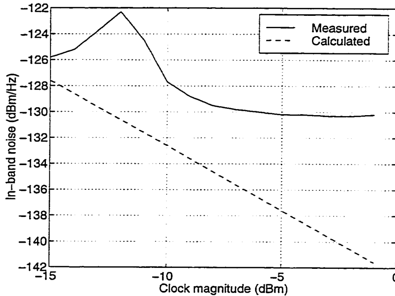
Figure 7.48: Measured in-band noise as a function of clock magnitude.
