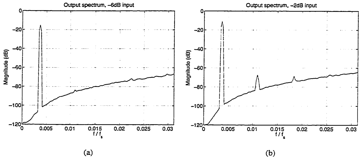
Figure 2.15: Increase in baseband harmonics for inputs near full scale: (a) -6\text{dB} input, (b) -2\text{dB} input.
