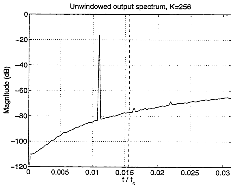
Figure 2.11: Unwindowed averaged periodogram near dc.
