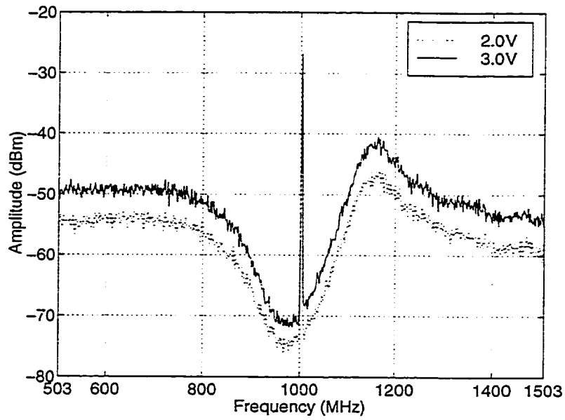
Figure 7.41: Varying V_{BUF} .
