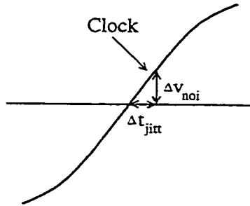
Figure 7.47: Clock jitter caused by circuit noise.
