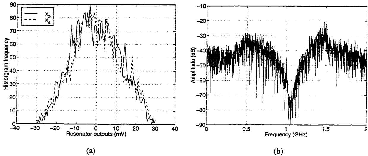
Figure 7.57: Scaled DAC currents k_{n2} = k_{n4} = 500\mu\text{A} : (a) resonator output histograms, (b) output spectrum.
