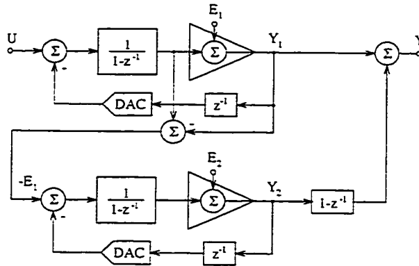
Figure 2.8: A multistage \Delta\Sigma M.
