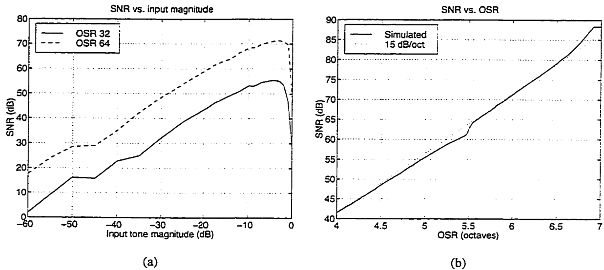
Figure 2.14: Performance of ideal double integration \Delta\Sigma .
