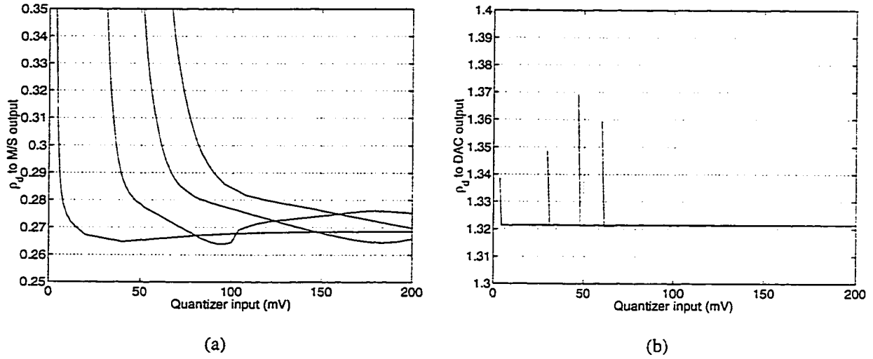
Figure 7.23: ZCT characteristics for (a) M/S latch output, (b) one-sample delayed output.
