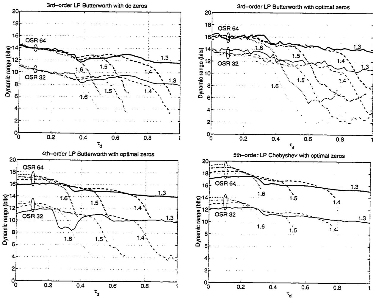
Figure 4.19: Dynamic range for high-order LP CT \Delta\Sigma Ms. Numbers on curves are OOBG values.
