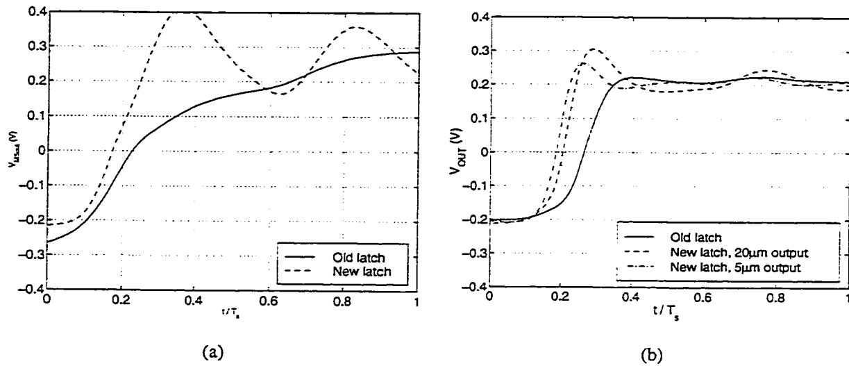
Figure 7.52: Output waveforms: (a) M/S latch, (b) output buffer.
