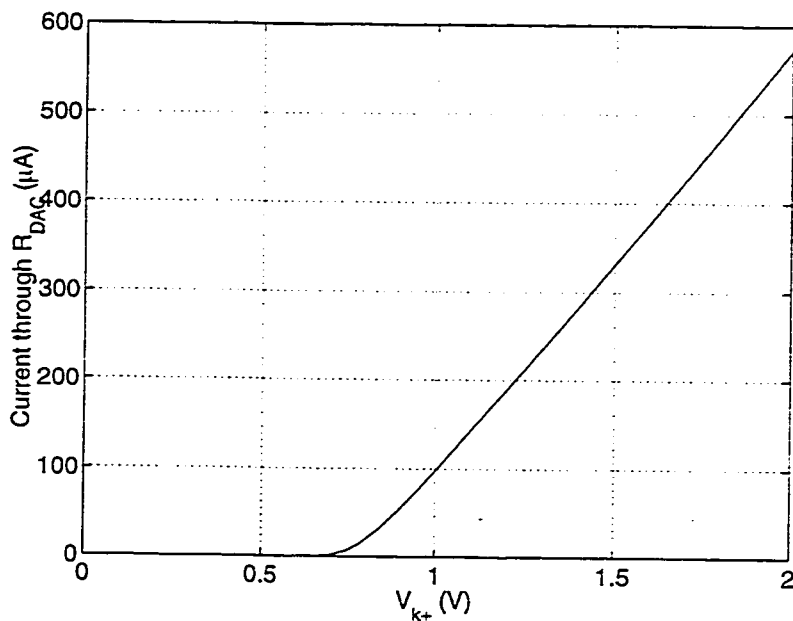
Figure B.4: DAC current vs. control voltage.
