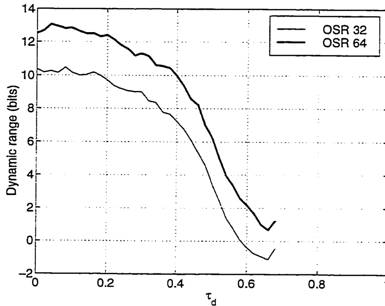
Figure 4.10: Dynamic range for double integration CT \Delta\Sigma M.
