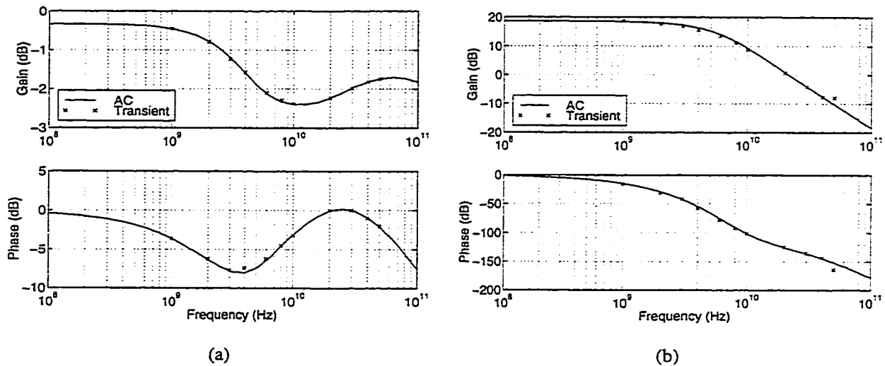
Figure 7.22: Original preamp ac analyses: (a) input follower, (b) entire circuit.
