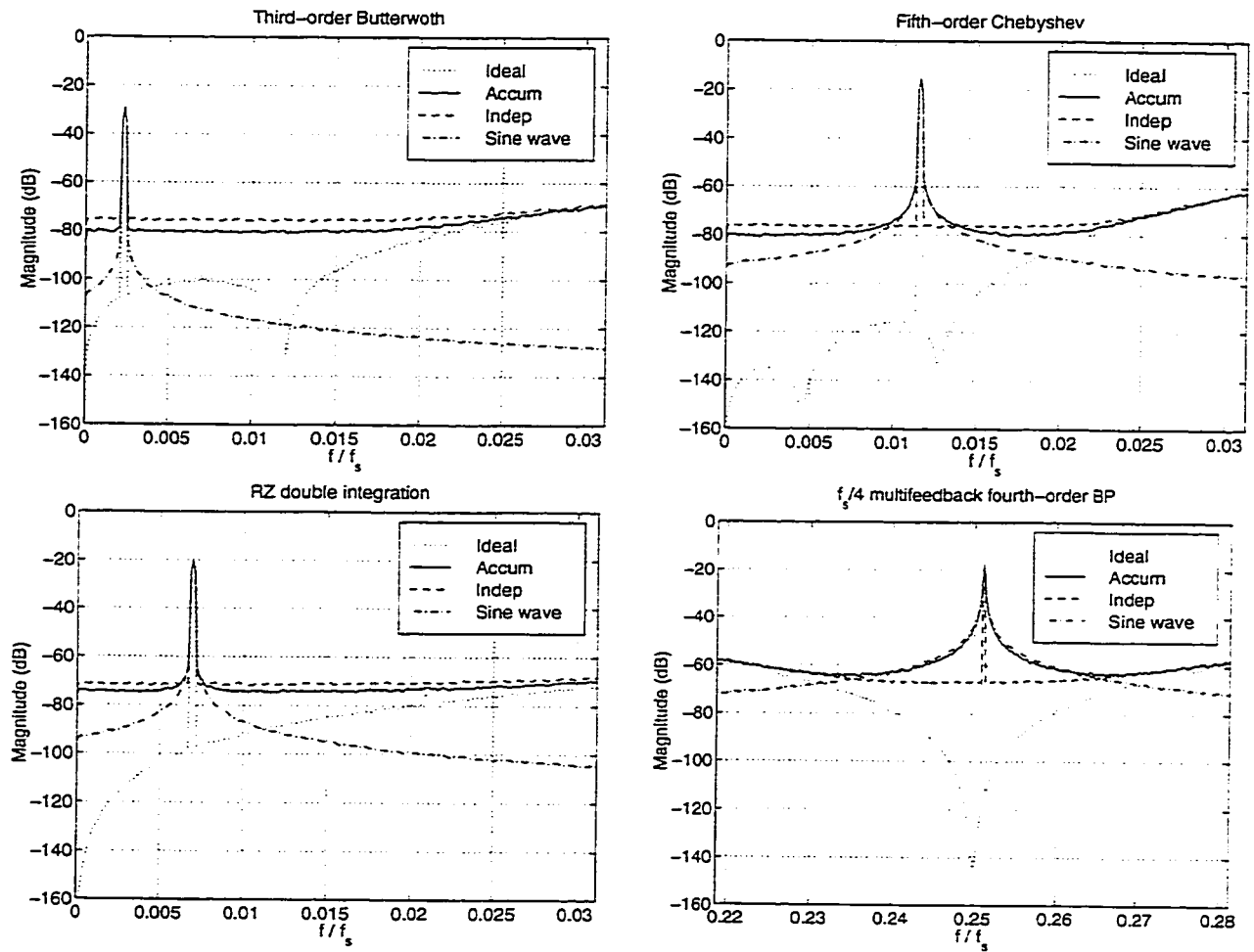
Figure 5.9: Comparison of \Delta\Sigma M spectra for independent and accumulated jitter, including spectrum of single tone at output of jittered S/H.
