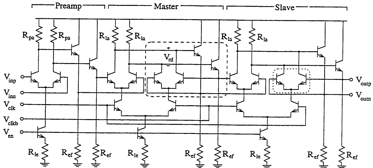
Figure 6.5: Typical high-speed CT \Delta\Sigma M master-slave latched comparator with preamplifier.
