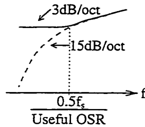
Figure 3.3: Ideal vs. real spectra in double integration modulators.
