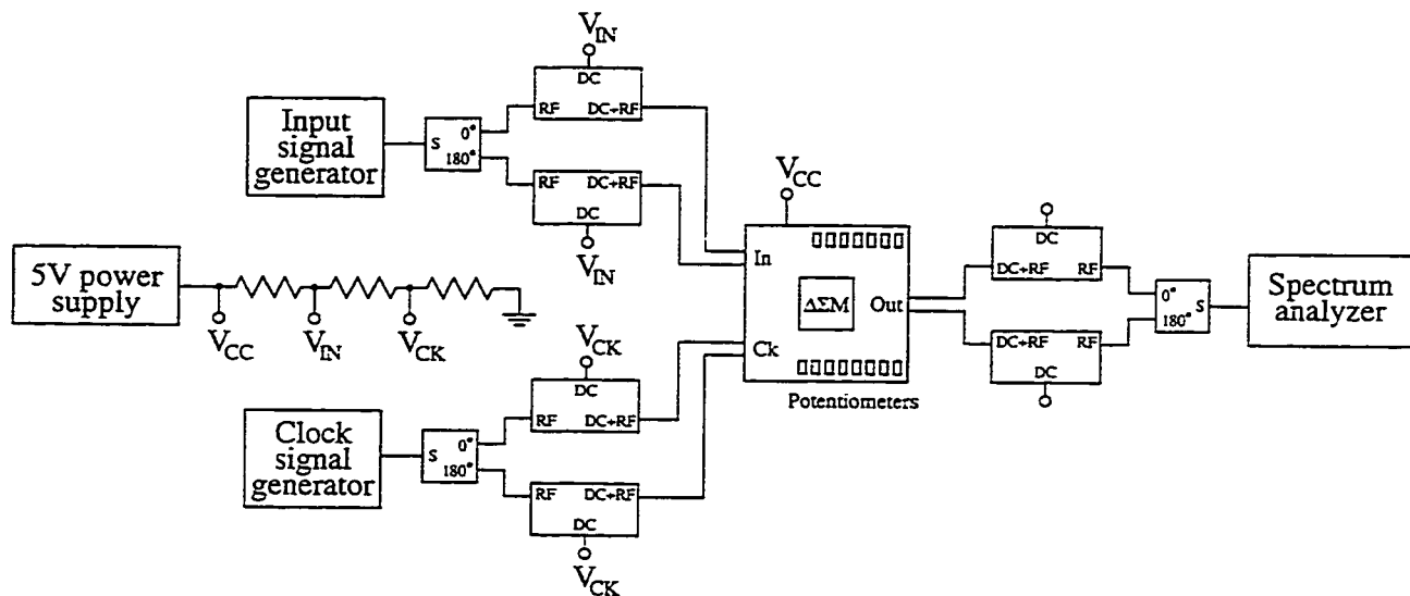
Figure 7.31: Measurement test setup.
