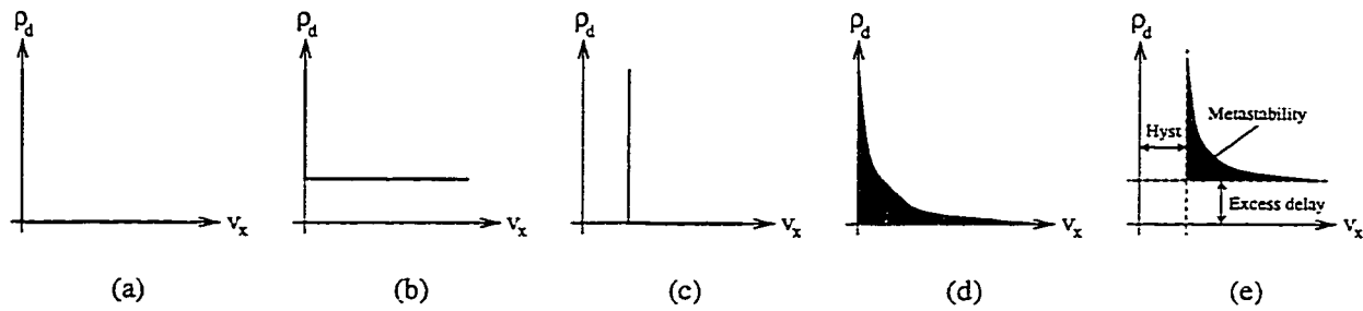
Figure 6.11: Quantizer characteristics: (a) ideal, (b) excess delay, (c) hysteresis, (d) metastability, (e) practical. Metastability severity is proportional to the area of the shaded region.
