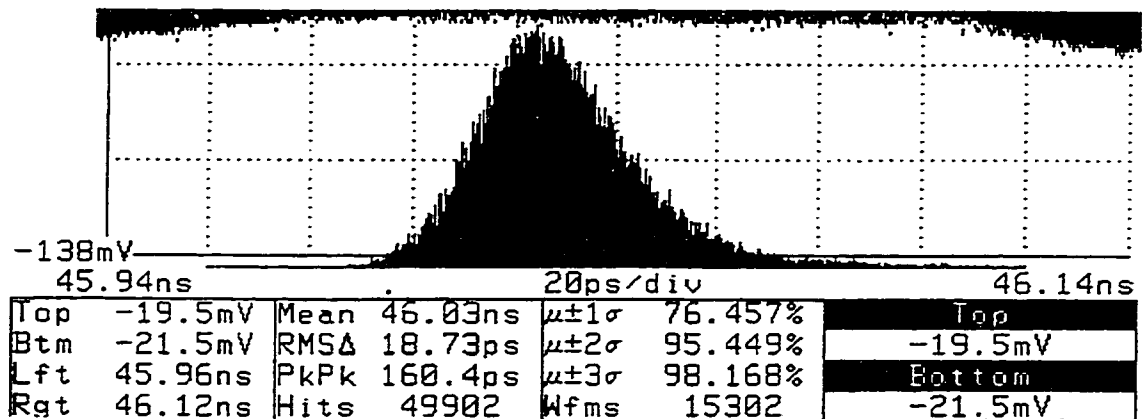
Figure 7.39: Histogram of time-domain output bit zero crossings.
