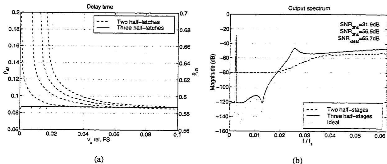
Figure 6.20: (a) Quantizer metastability curves and (b) output spectrum for quantizer with an additional latching stage.
