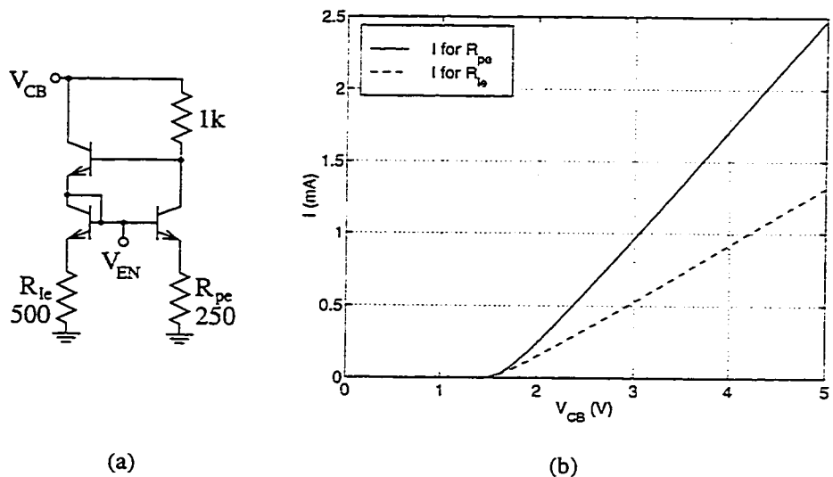
Figure B.3: (a) V_{EN} bias circuit, (b) current through bias transistor emitter resistors.
