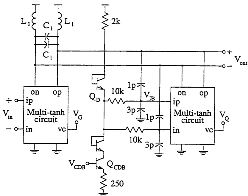
Figure 7.17: Band pass resonator block.
