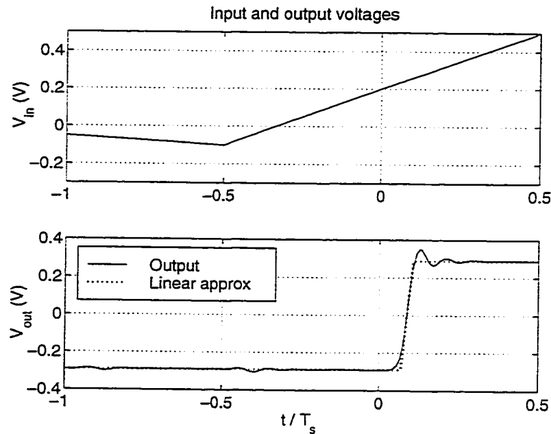
Figure 6.7: SPICE input and output waveforms with linear approximation to output.
