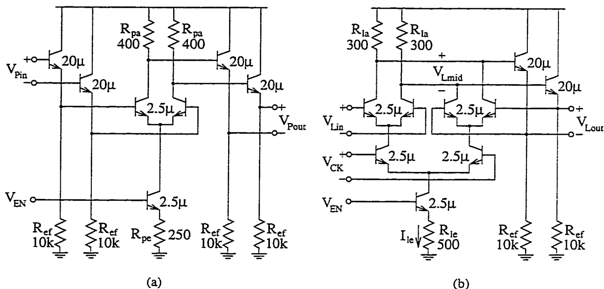
Figure 7.21: Schematics for (a) preamplifier, (b) half-latch.
