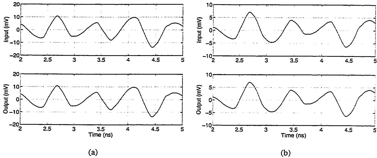
Figure 7.50: (a) First and (b) second resonator output buffer waveforms.
