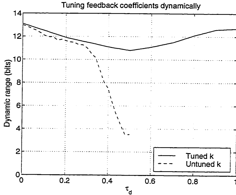
Figure 4.23: Multi-feedback BP modulator dynamic range with k tuning.
