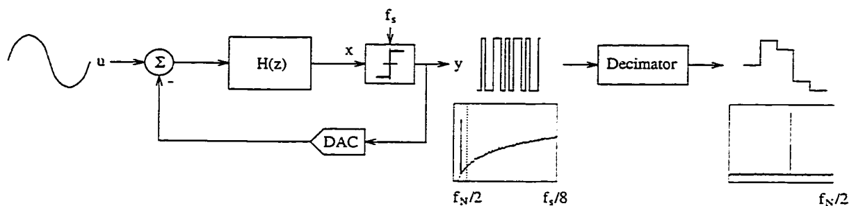
Figure 2.5: Complete \Delta\Sigma ADC block diagram including decimator.
