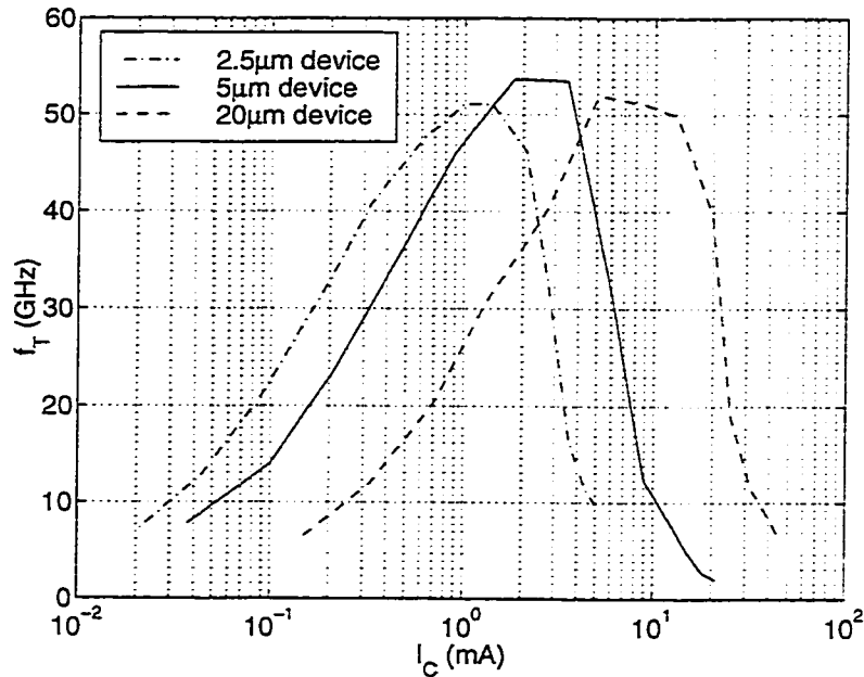
Figure 7.49: Measured f_T vs. I_C curves for SiGe BJTs.
