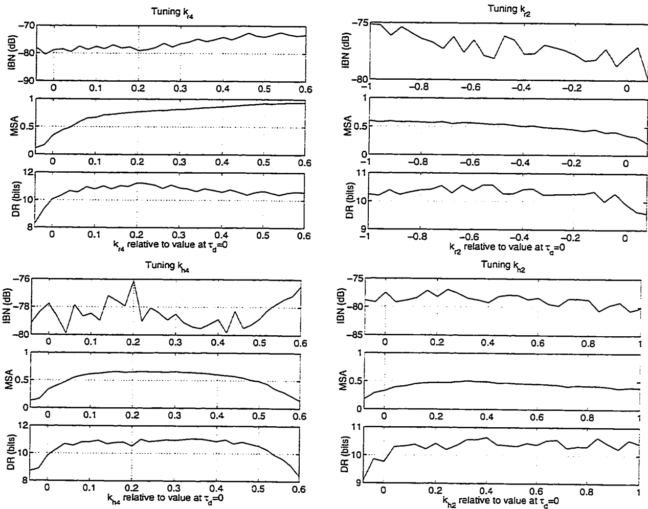
Figure 4.22: Fourth-order f_s/4 BP CT \Delta\Sigma performance at \rho_d = 35\% delay with feedback coefficient tuning.
