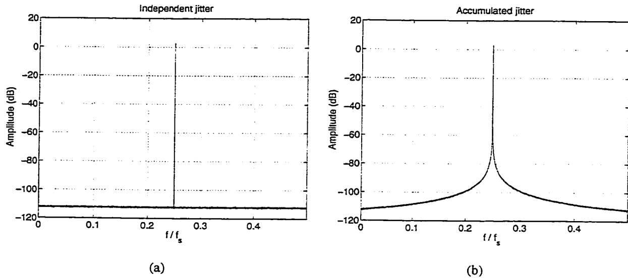
Figure 5.7: Unwindowed spectra of sine wave carriers sampled with jitter: (a) independent jitter, (b) accumulated jitter.
