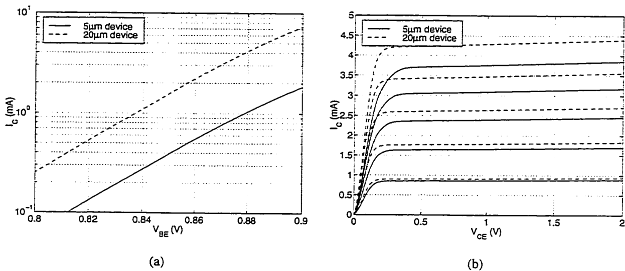
Figure B.1: BJT characteristics: collector current vs. (a) V_{BE} , (b) V_{CE} .
