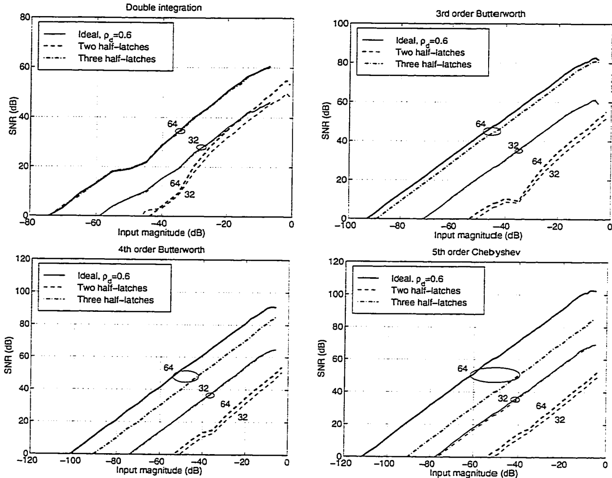
Figure 6.21: Dynamic range plots. Numbers on curves are OSR values.
