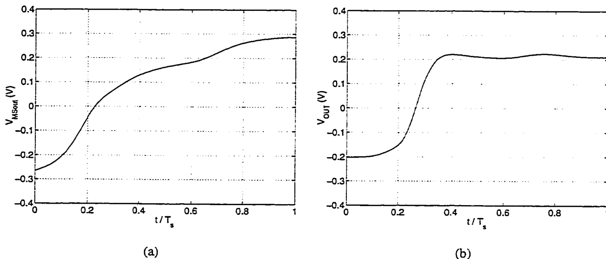
Figure 7.25: Output waveforms: (a) M/S latch, (b) output buffer.
