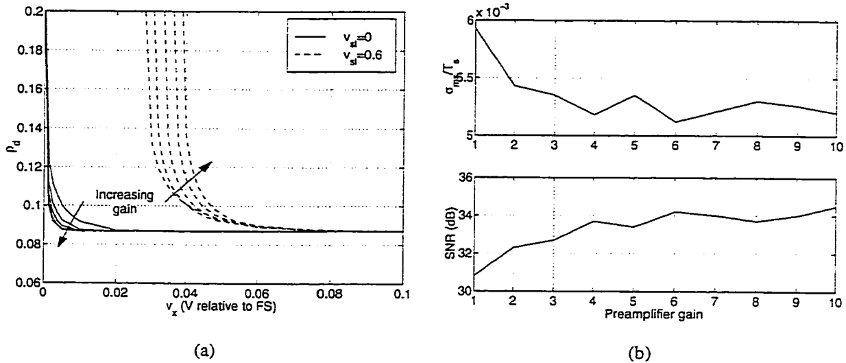
Figure 6.19: (a) Quantizer metastability curves and (b) modulator performance as a function of preamplifier gain.
