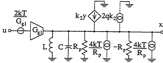
Figure 7.4: Input transconductor equivalent circuit for noise considerations.
