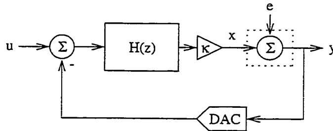
Figure 4.6: Linearized \Delta\Sigma M with one-bit quantizer arbitrary gain \kappa .
