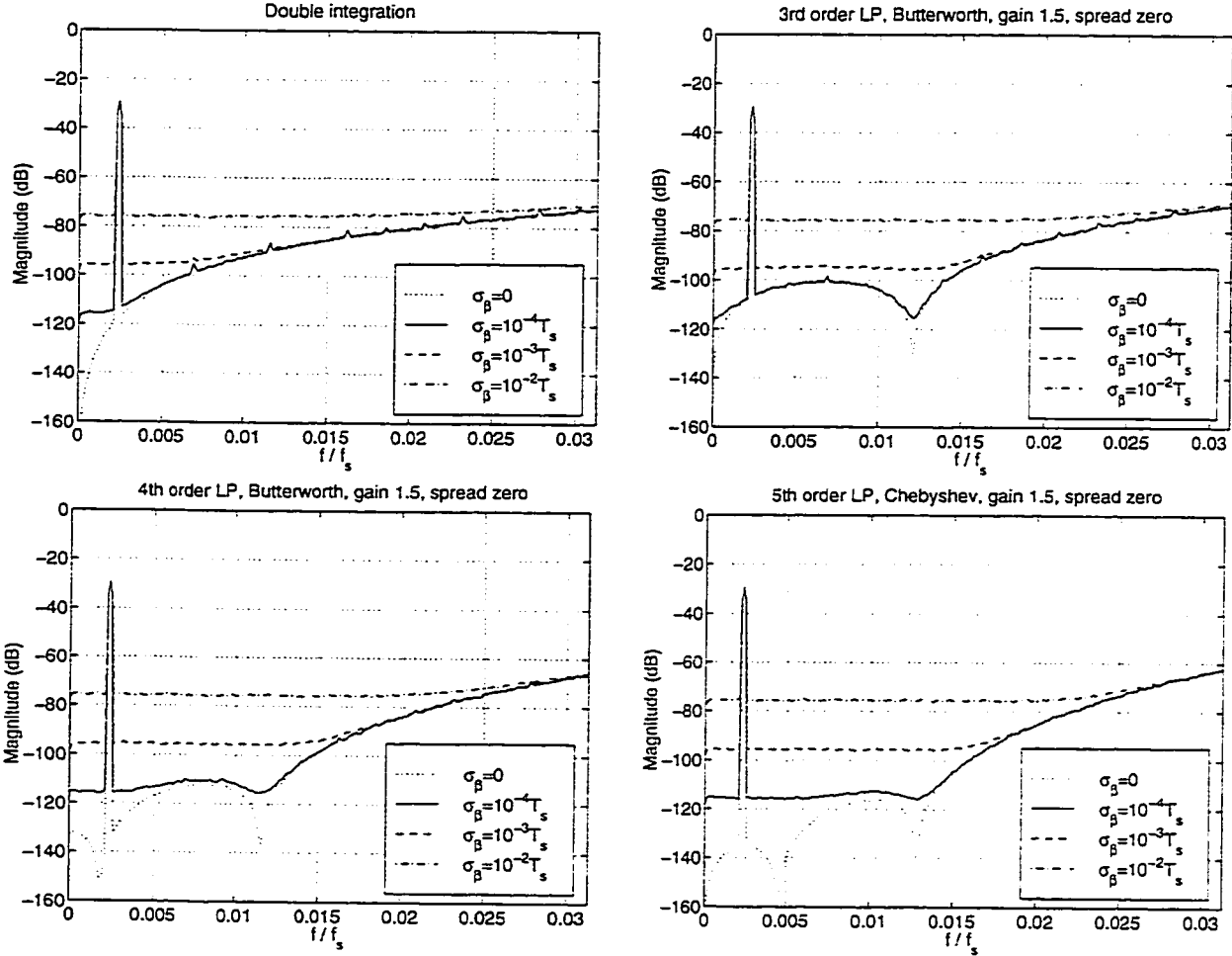
Figure 5.3: Output spectra for NRZ LP modulators with clock jitter.
