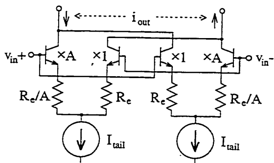
Figure 7.10: Multi-tanh circuit.
