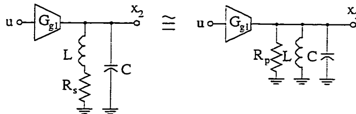
Figure 7.3: Series/parallel tank equivalence near resonance.
