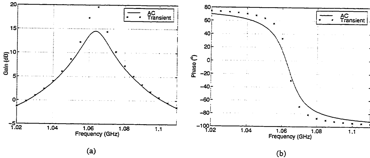
Figure 7.19: Transient analysis for V_G = 2.2V and V_Q = 2.6V : (a) gain, (b) phase.
