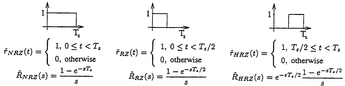
Figure 4.14: Common DAC pulse types.
