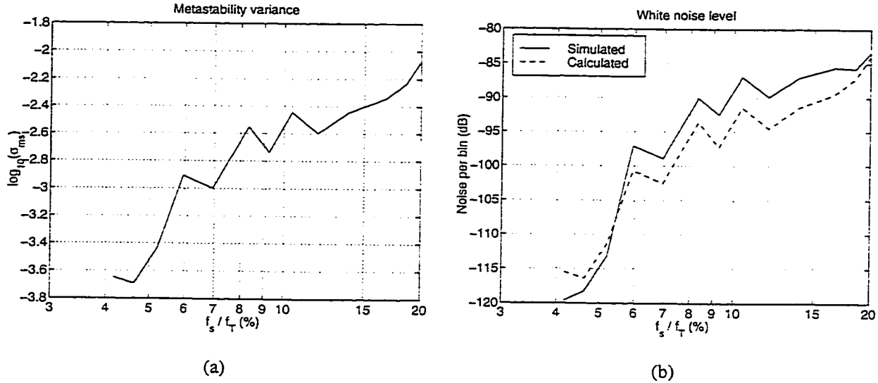
Figure 6.23: Effect of increasing f_s on (a) \sigma_{ms} , (b) calculated and simulated noise level.
