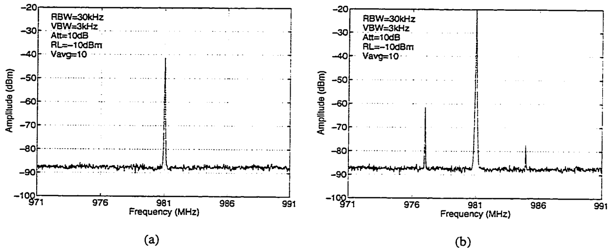
Figure 7.43: Measured modulator spectra: (a) V_{in} = -40\text{dBm} , (b) V_{in} = -20\text{dBm} .
