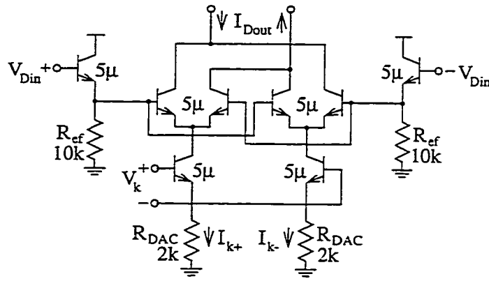
Figure 7.26: Current-steering DAC schematic.
