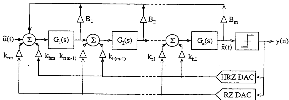
Figure 5.2: Block diagram for general CT \Delta\Sigma M architecture.
