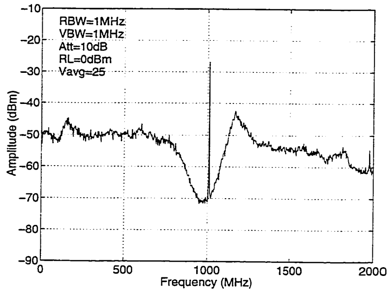
Figure 7.32: NRZ modulator output spectrum.
