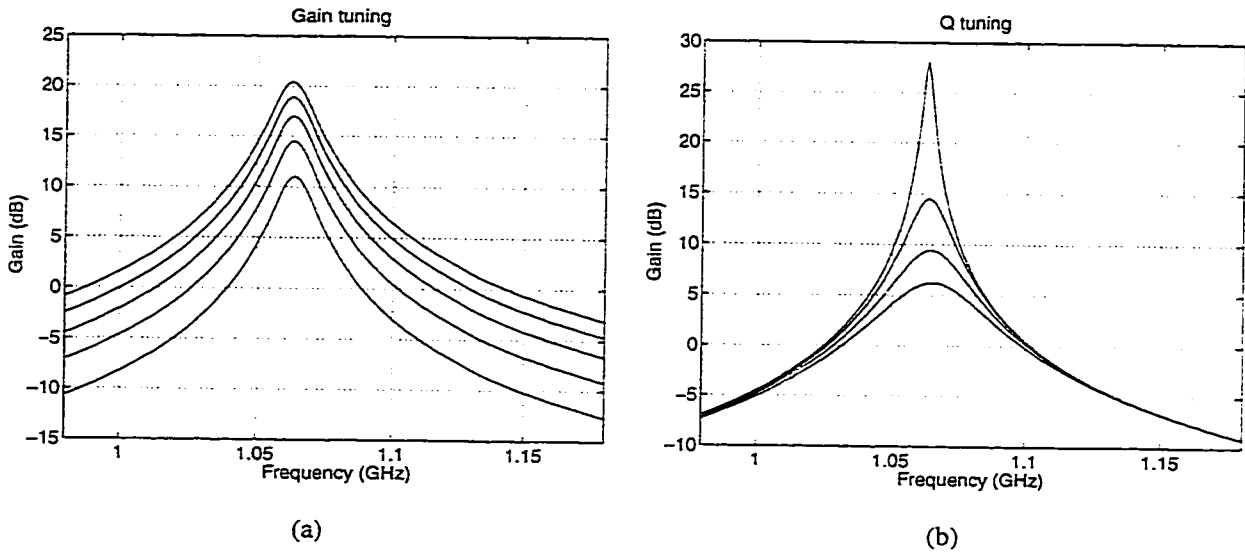
Figure 7.18: Filter gain characteristic: (a) fixed V_Q = 2.6V , stepping V_G by 0.2V from 2.0V to 2.8V, (b) fixed V_G = 2.2V , stepping V_Q by 0.1V from 2.4V to 2.7V.
