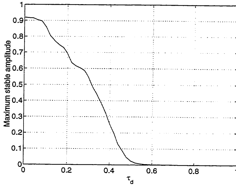
Figure 4.9: Maximum stable amplitude for double integration CT \Delta\Sigma\text{M} .
