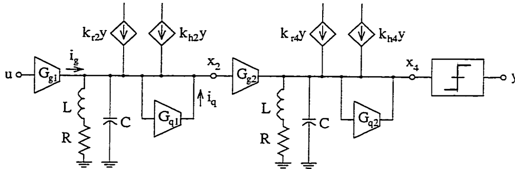
Figure 7.2: Approximate single-ended model for modulator.
