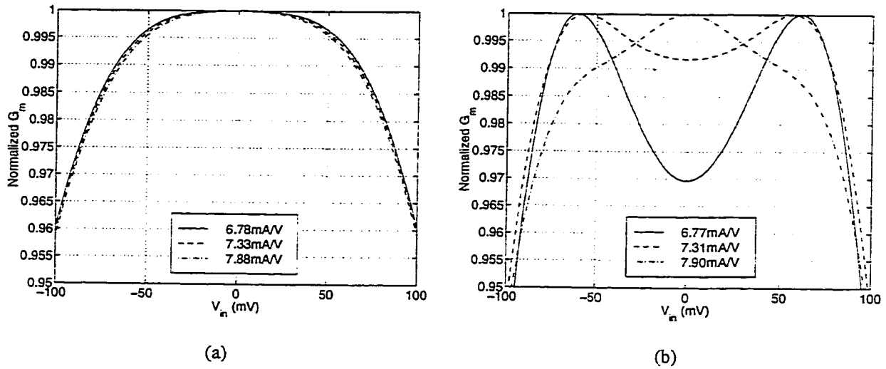
Figure 7.15: Linearity for emitter diodes vs. emitter resistors: (a) A = 4 , D = 3 , (b) A = 8 , R_e = 100\Omega .
