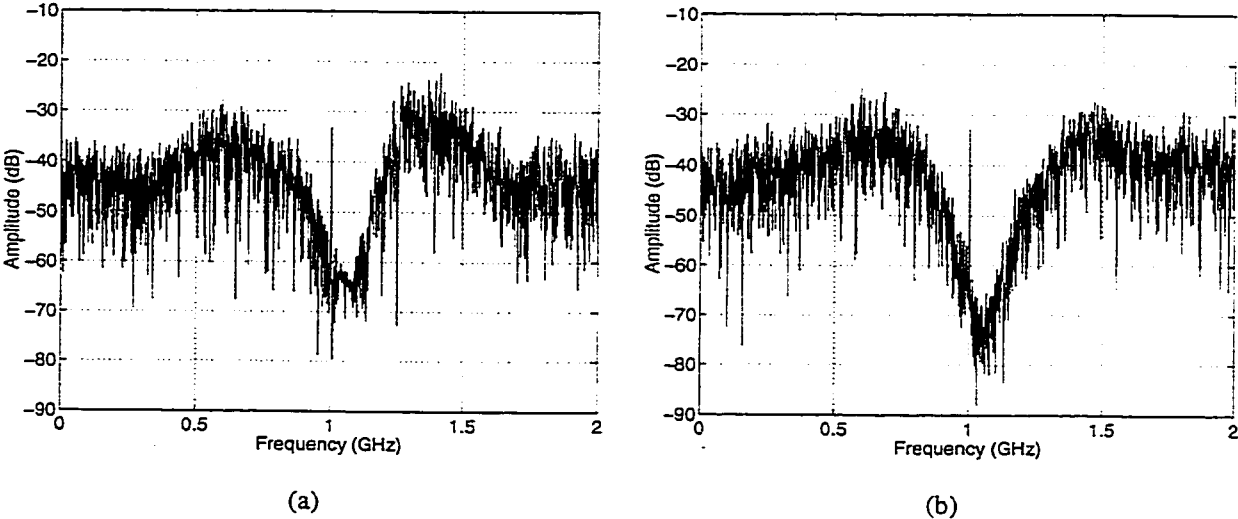
Figure 7.55: SPICE output spectra for (a) original modulator, (b) optimized modulator.
