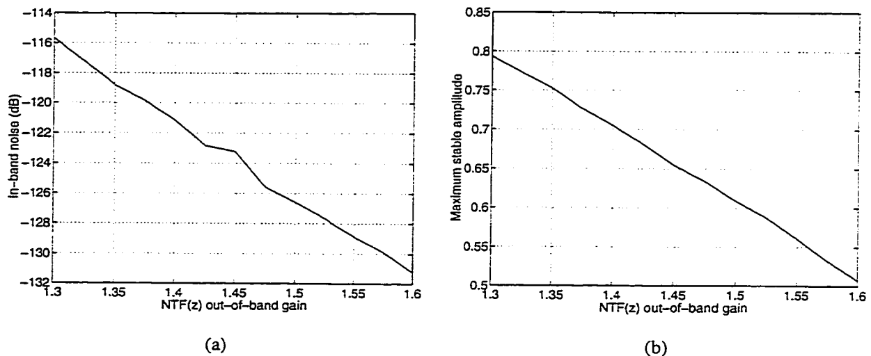
Figure 4.18: Effect of out-of-band-gain on fifth-order Chebyshev modulator: (a) IBN, (b) MSA.
