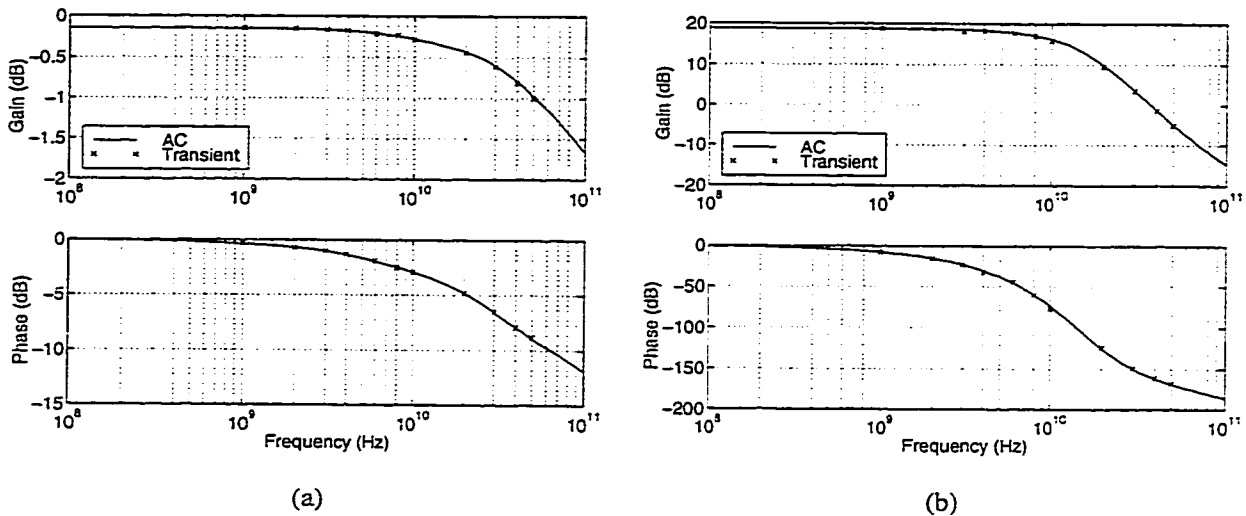
Figure 7.51: Optimized preamp ac analyses: (a) input follower, (b) entire circuit.
