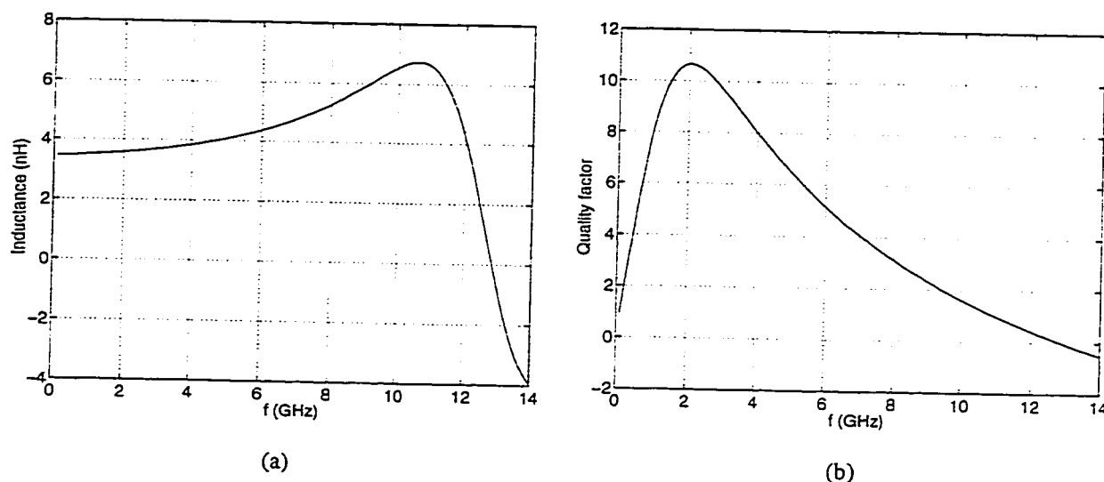
Figure 7.7: SPICE ac analysis of inductor: (a) L , (b) Q .
