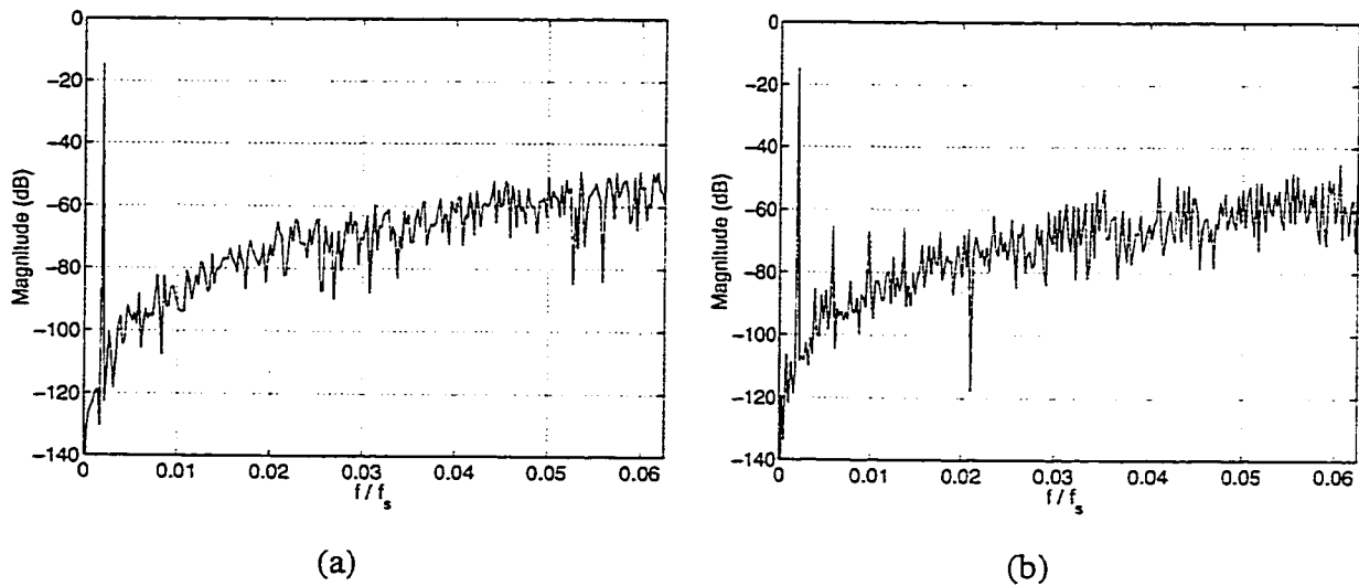
Figure 3.2: Output spectra using op amps with (a) no slew-rate limiting, (b) slew-rate limiting.
