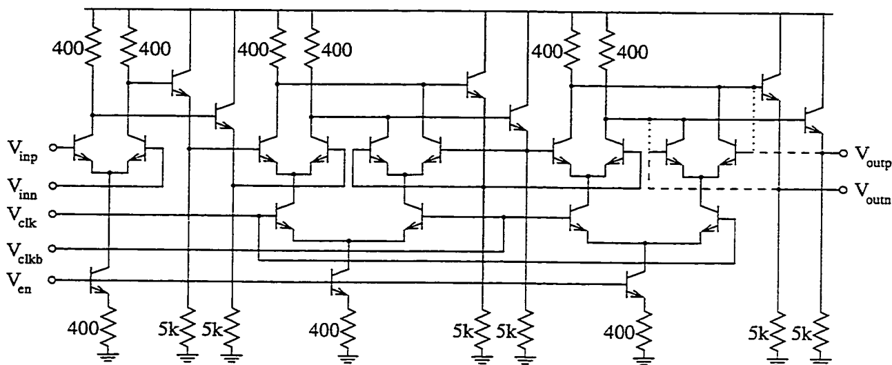
Figure 4.15: ECL-style latched comparator with preamplification for enhanced resolution at high speed. For an NRZ comparator, connect the final differential pair via the dashed lines; for RZ, connect the dotted lines instead.
