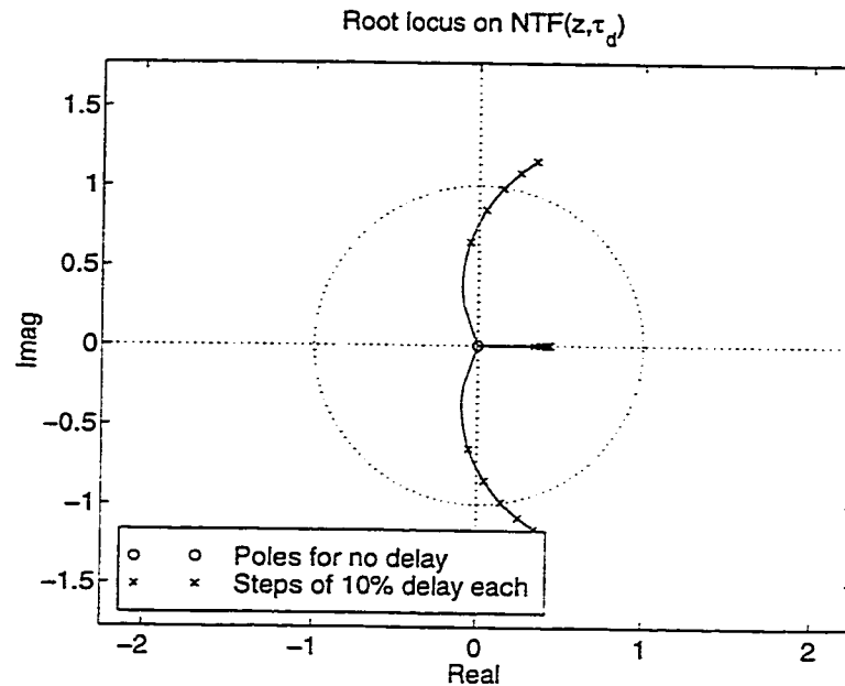
Figure 4.7: Effect of loop delay on root locus of NTF(z, \tau_d) .
