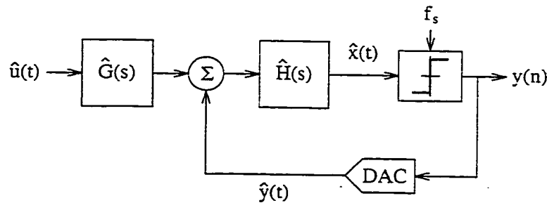
Figure 4.2: General CT \Delta\Sigma block diagram.
