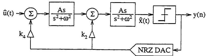
Figure 4.12: Block diagram for BP CT \Delta\Sigma M with integrators replaced by resonators that cannot implement desired equivalent H(z) .
