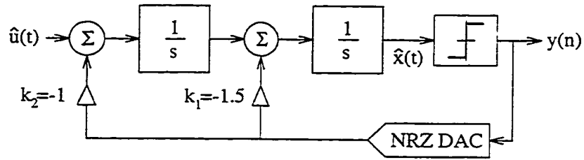
Figure 4.11: Block diagram for LP CT \Delta\Sigma M from Figure 4.1.
