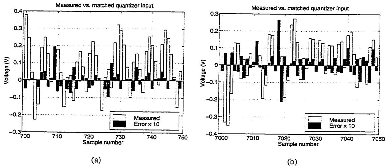
Figure 6.2: Examples of z -domain extraction from SPICE data.
