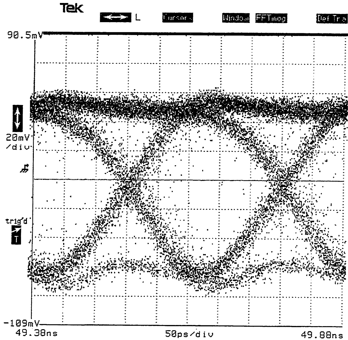
Figure 7.38: Output bit stream eye diagram.
