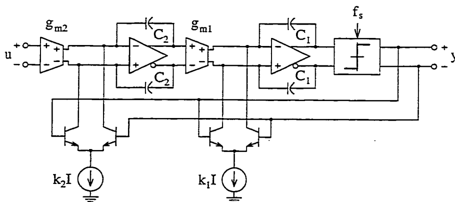
Figure 2.16: InP second-order CT \Delta\Sigma M by Jensen et al.
