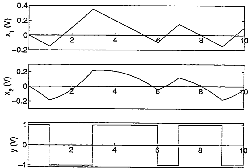
Figure 3.1: Typical integrator output and quantizer waveforms.
