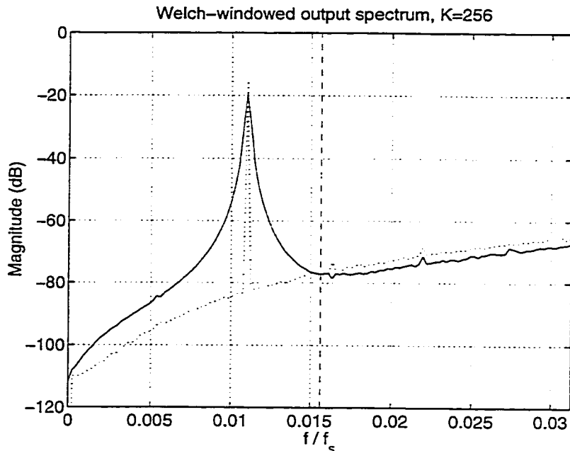
Figure 2.13: Welch-windowed averaged periodogram near dc.
