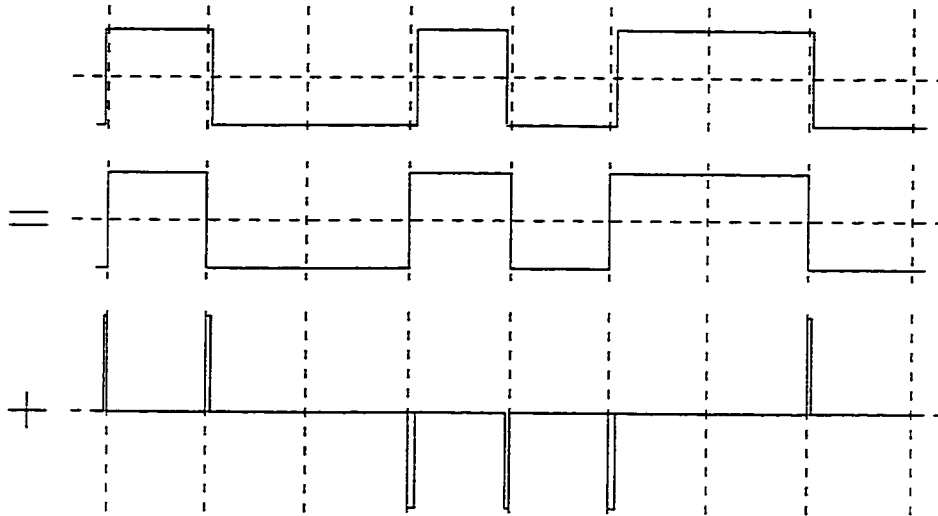
Figure 5.4: Equivalent representations of a jittered bit stream.
