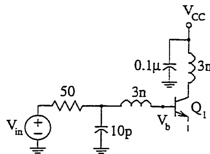
Figure 7.46: Model of actual circuit input.
