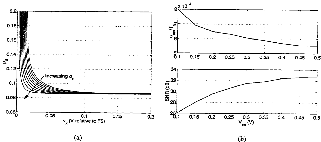
Figure 6.16: (a) Quantizer metastability curves and (b) modulator performance as a function of \sigma_x .
