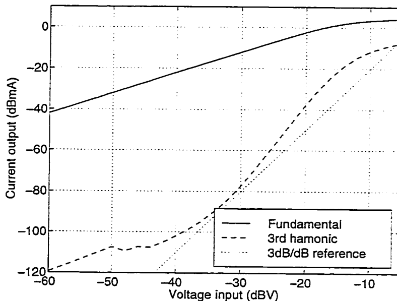
Figure 7.16: Linearity plot for a multi-tanh circuit.
