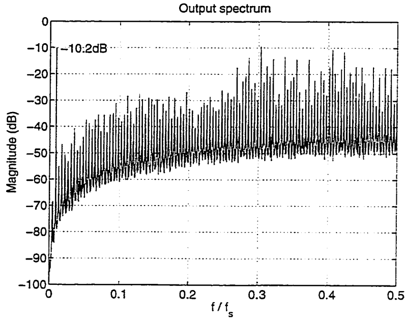
Figure 2.4: Simulated output bit stream power spectrum.
