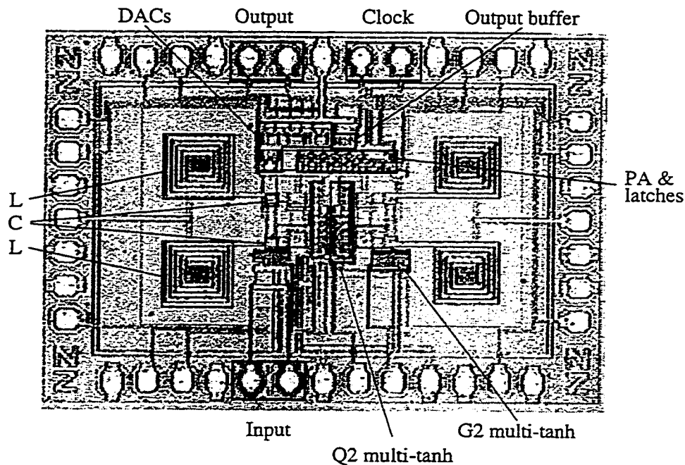
Figure 7.30: Die photomicrograph of NRZ modulator.
