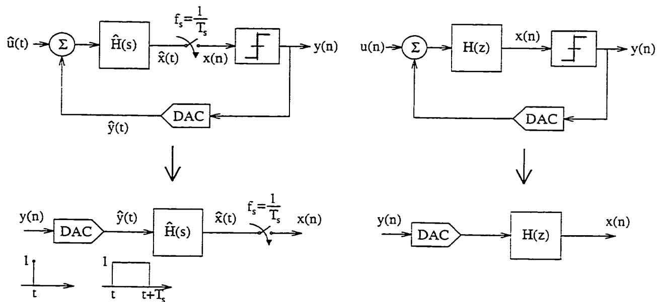
Figure 4.3: Open-loop CT \Delta\Sigma\text{M} and its DT equivalent.
