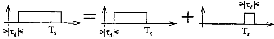
Figure 4.5: Delayed NRZ pulse as a linear combination.
