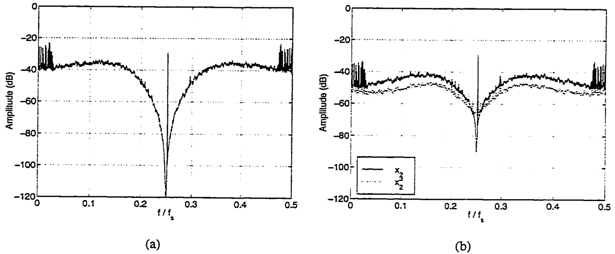
Figure 7.5: Spectrum of (a) output bits, (b) x_2 and x_2^3 .
