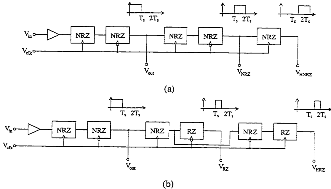
Figure 7.20: Overall latching scheme and waveforms: (a) NRZ modulator, (b) RZ modulator.
