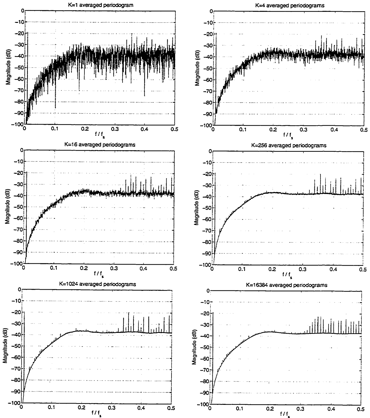
Figure 2.10: Effect of averaging on spectrum variance.
