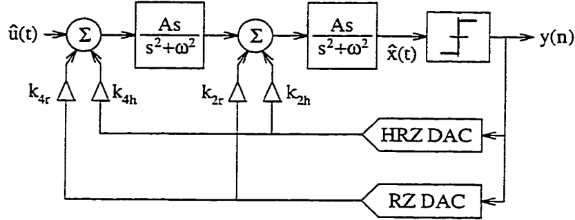
Figure 4.13: Multi-feedback BP CT \Delta\Sigma M architecture.
