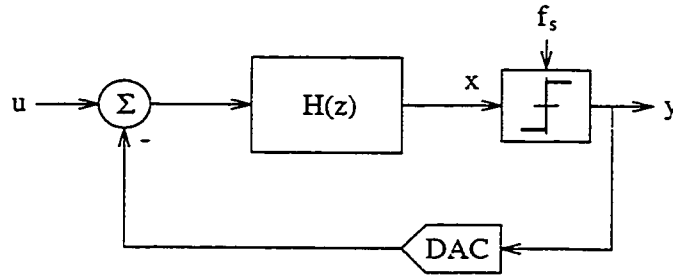
Figure 2.1: Basic components of a \Delta\Sigma M for ADC.
