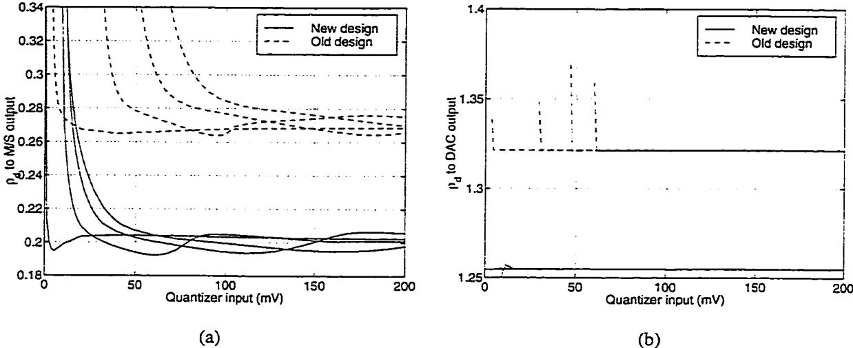
Figure 7.54: New ZCT characteristics for (a) M/S latch output, (b) one-sample delayed output.
