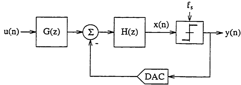
Figure 2.17: A general DT \Delta\Sigma M including input prefiltering.
