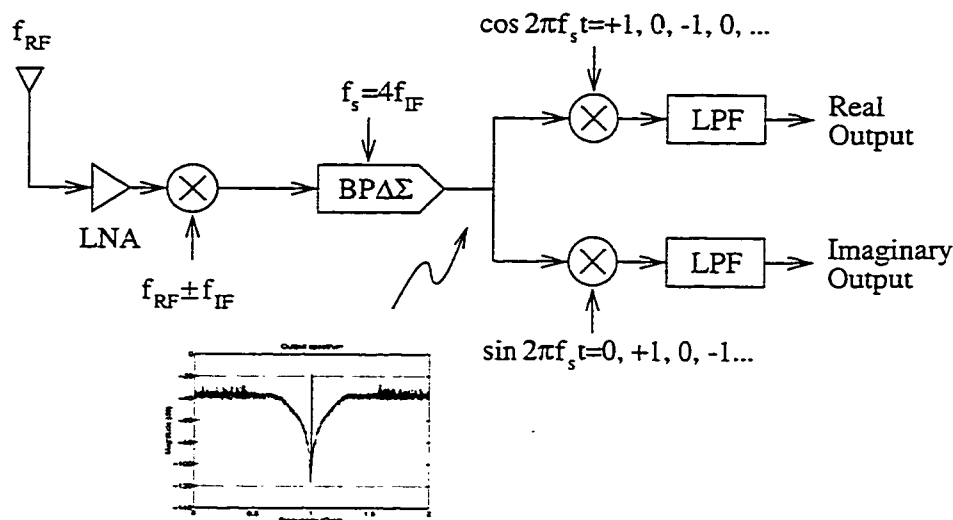
Figure 2.7: Typical radio receiver application for a band pass \Delta\Sigma .
