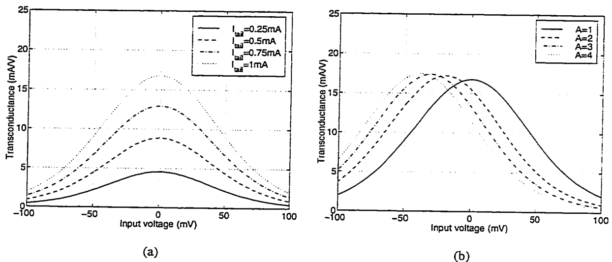
Figure 7.9: Transconductance of differential pair as a function of (a) tail current, (b) number of transistors.
