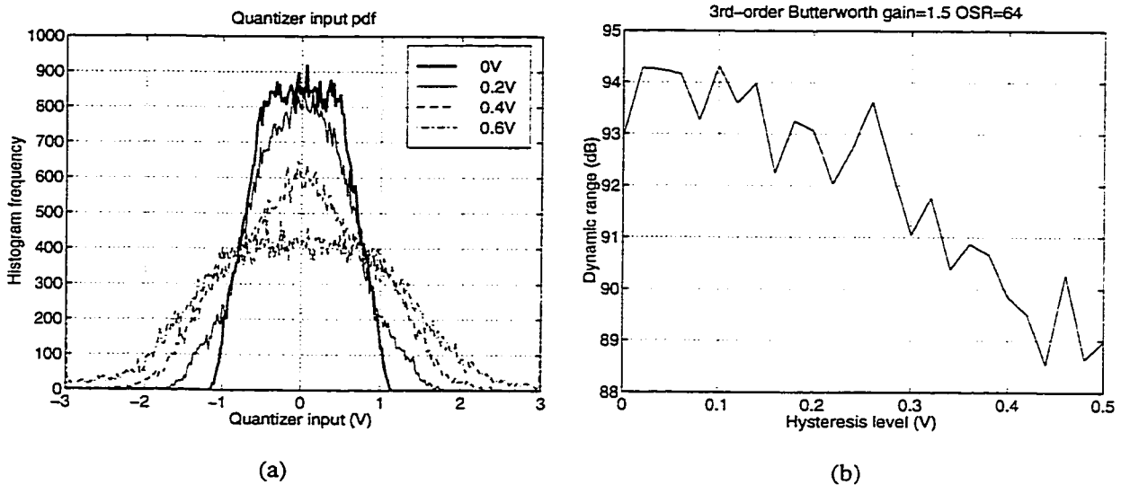
Figure 6.12: Quantizer hysteresis in third-order Butterworth modulator: (a) quantizer input pdf, (b) modulator dynamic range.
