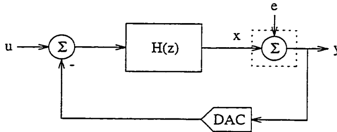
Figure 2.2: Linearizing the quantizer in a \Delta\Sigma M.
