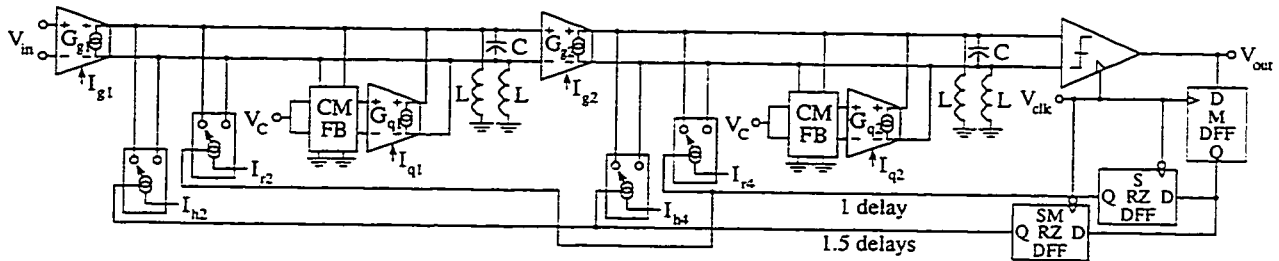
Figure 7.1: A 4GHz fourth-order BP CT \Delta\Sigma\text{M} .
