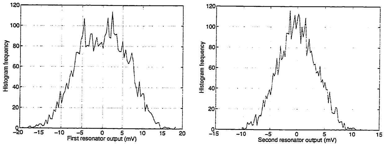
Figure 7.56: Resonator output voltage histograms from SPICE.
