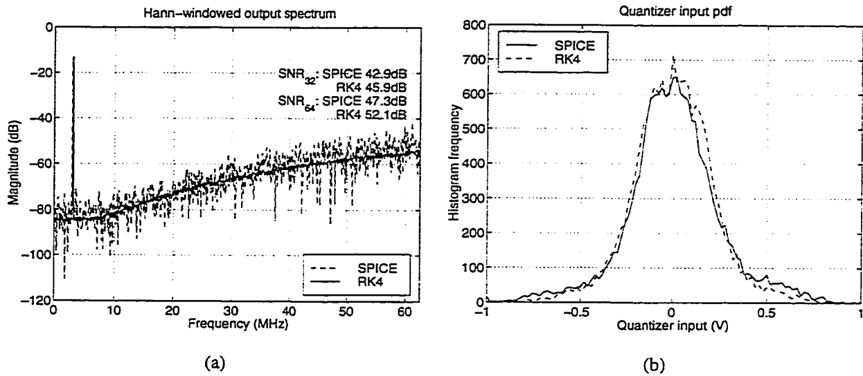
Figure 6.9: Comparison of SPICE and Runge-Kutta simulation programs: (a) output spectra, (b) quantizer input pdfs.
