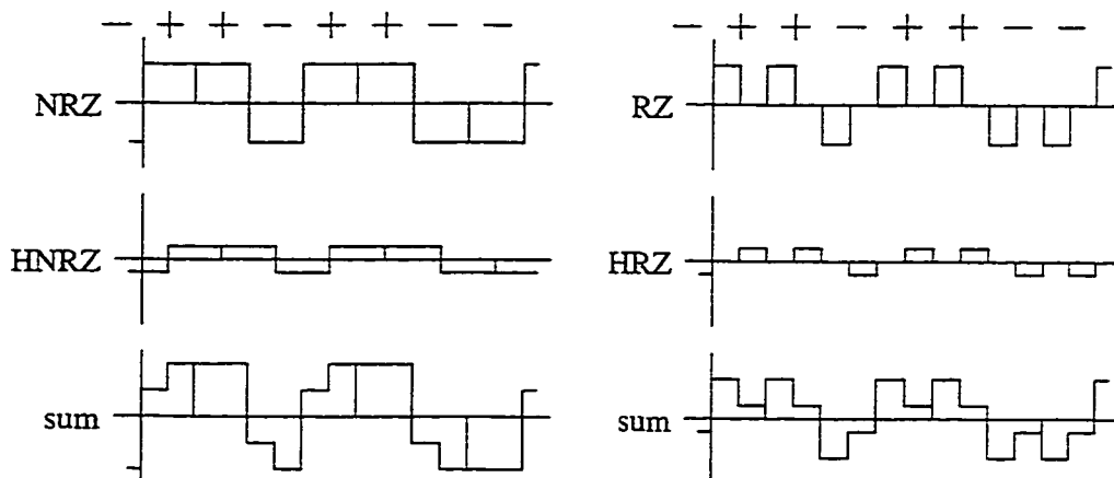
Figure 7.45: Illustration of nonuniform feedback caused by a half-delayed NRZ DAC.
