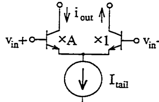
Figure 7.8: Differential pair transconductor.
