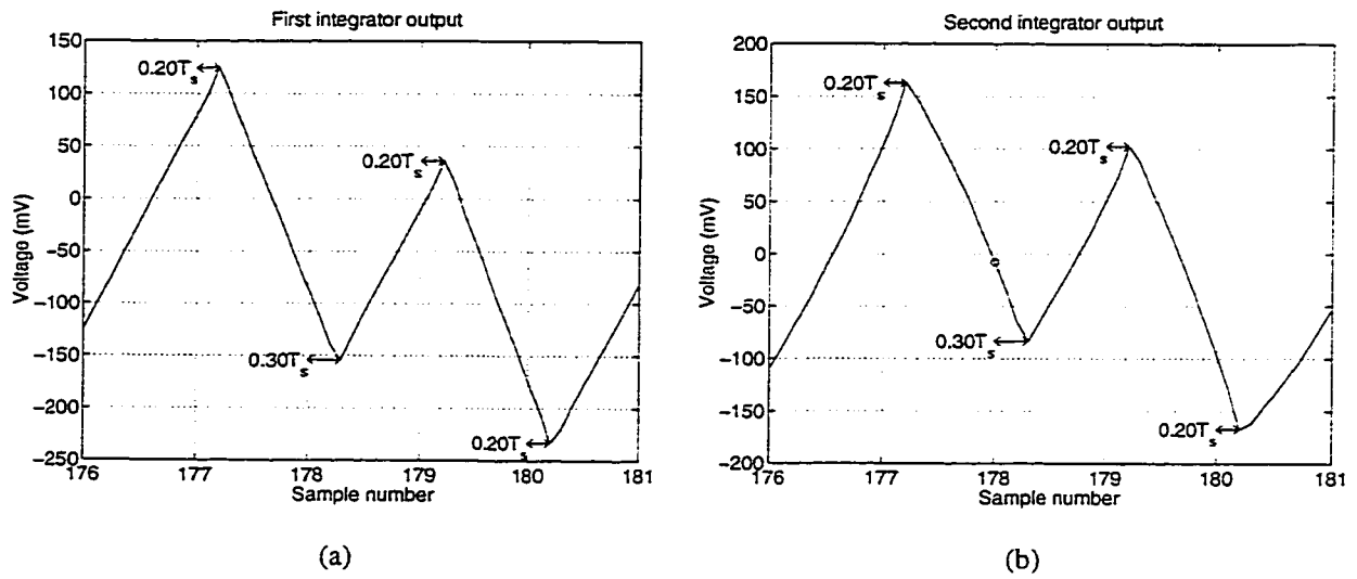
Figure 6.3: First and second integrator output waveforms from SPICE showing additional excess delay at sample 178.
