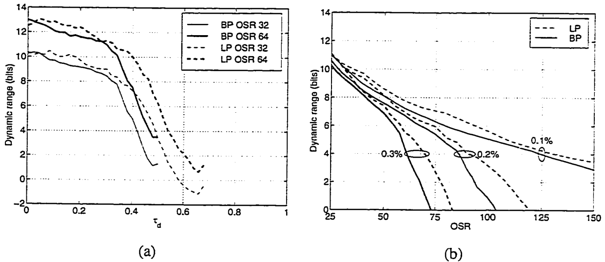
Figure 4.16: (a) Dynamic range for multi-feedback BP CT \Delta\Sigma M, with comparison to double integration results. (b) Same graph with OSR as independent variable; numbers on curves are \tau_d \times f_N .
