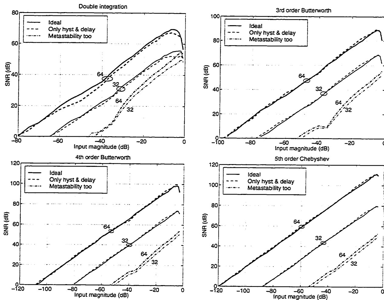
Figure 6.14: Dynamic range plots. Numbers on curves are OSR values.
