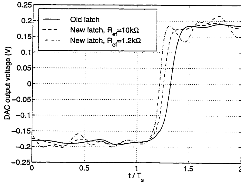
Figure 7.53: Dynamic DAC output voltage.
