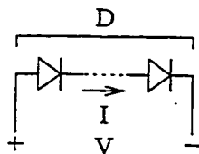
Figure 7.14: Series-connected diodes.
