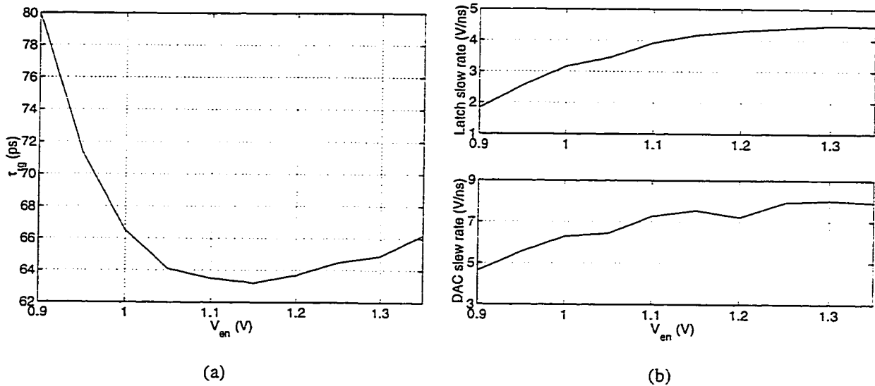
Figure 6.17: Effect of V_{en} on (a) regeneration time, (b) slew rates at latch output and DAC output.
