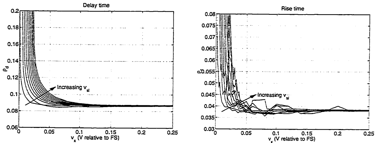
Figure 6.8: Example of numerically-characterized \rho_d and \rho_r values.
