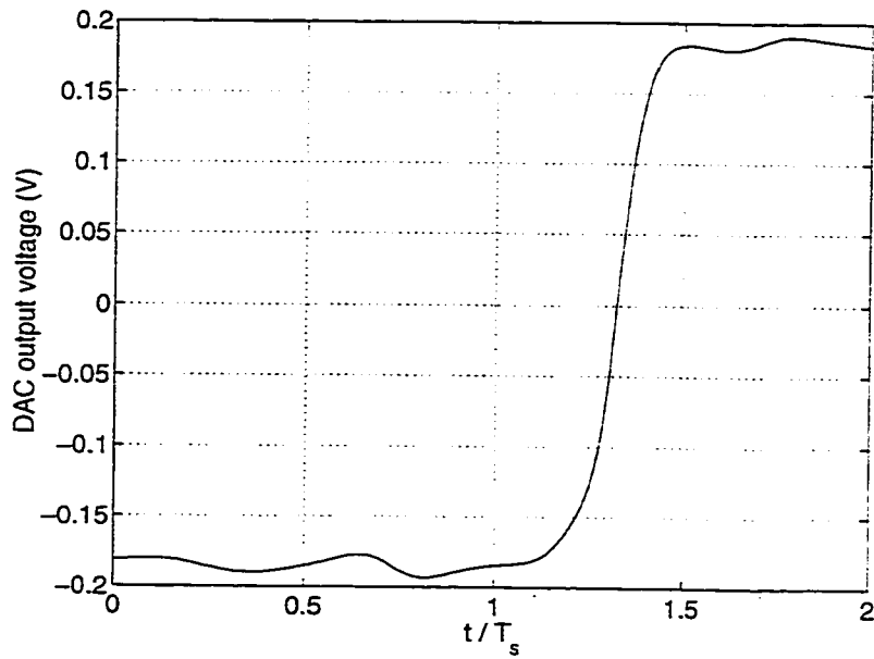
Figure 7.27: Dynamic DAC output voltage.
