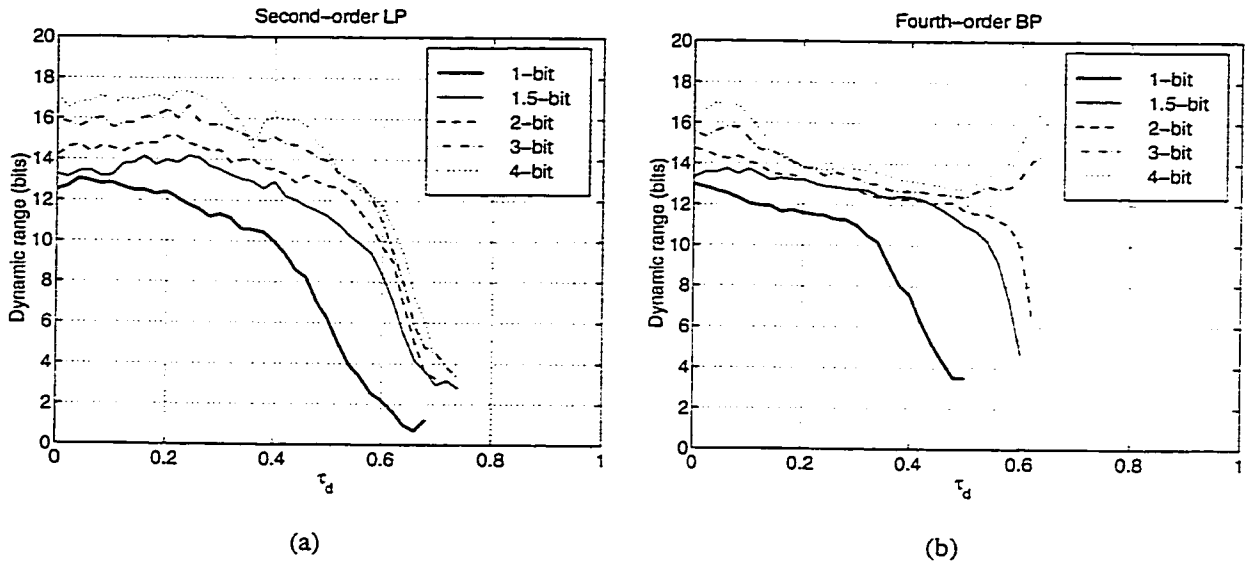
Figure 4.21: Modulators with multibit quantizers: (a) second-order LP, (b) fourth-order BP.
