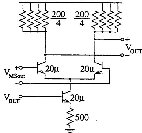
Figure 7.24: Modulator output buffer.
