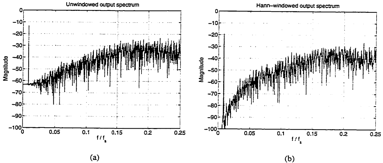
Figure 2.9: Effect of windowing: (a) unwindowed output spectrum, (b) windowed output spectrum.
