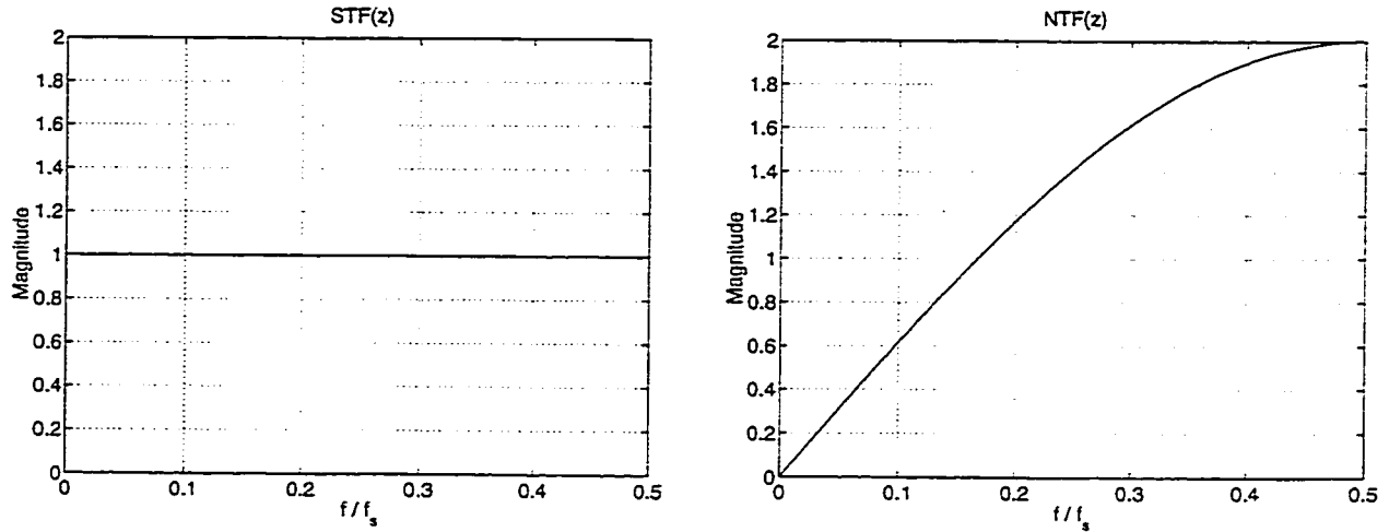
Figure 2.3: STF( z ) and NTF( z ) for circuit of Example 2.1.
