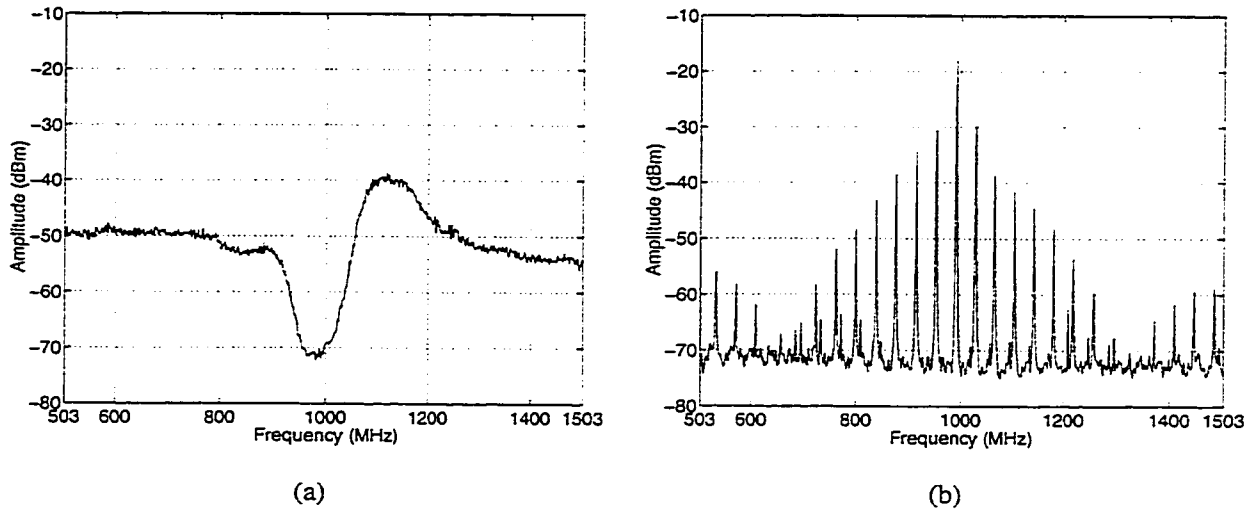
Figure 7.35: Oscillation in output spectrum: (a) V_Q = 3.31\text{V} , (b) V_Q = 3.33\text{V} .
