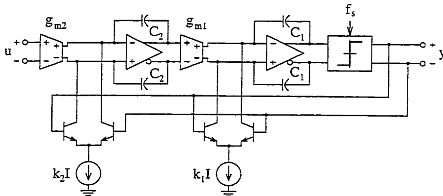
Figure 4.1: Example of high-speed double integration CT \Delta\Sigma M.
