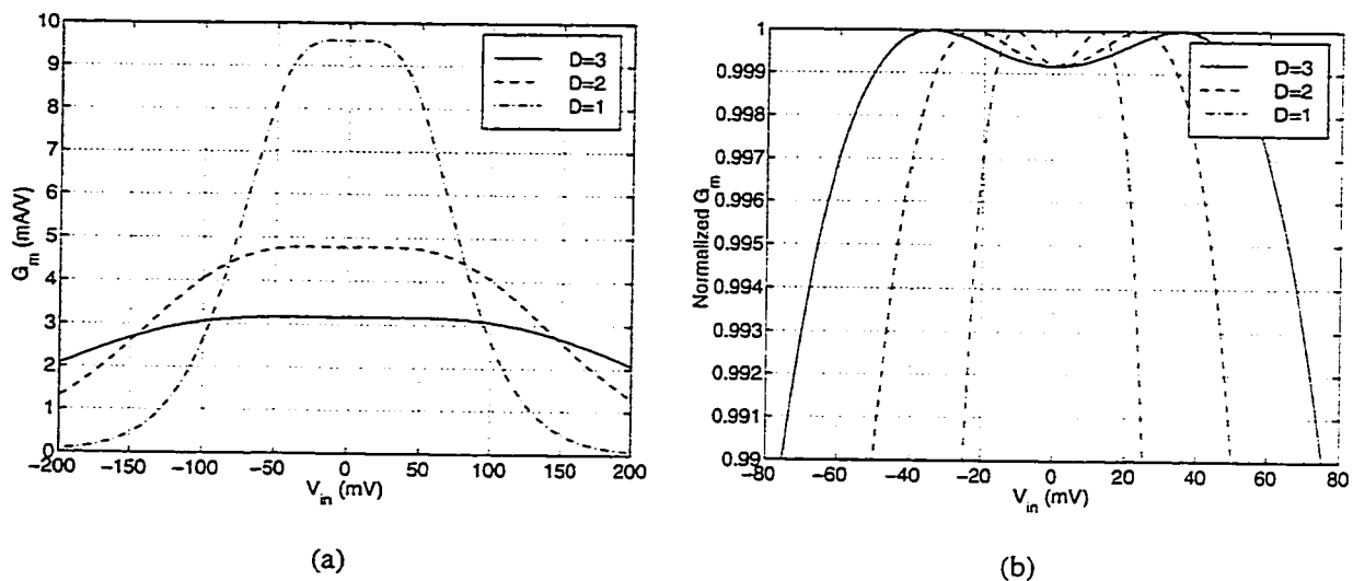
Figure 7.13: Transconductance as a function of number of diodes: (a) absolute, (b) normalized to peak G_g .
