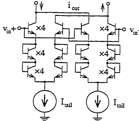
Figure 7.12: Actual transconductance topology used.
