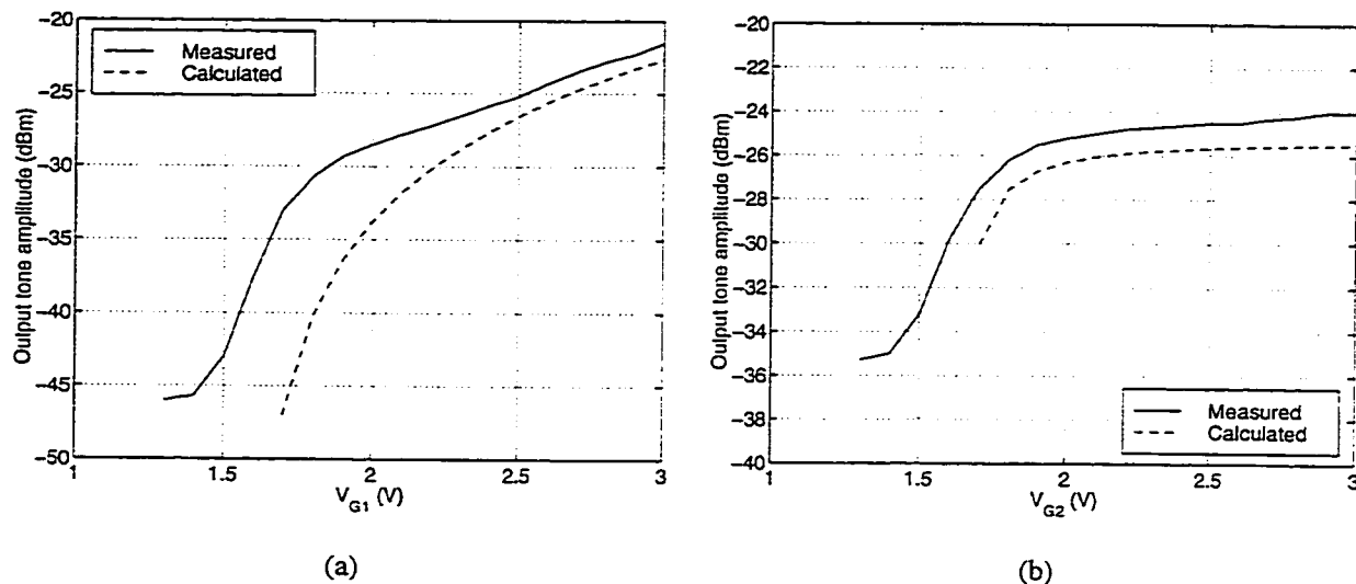
Figure 7.33: Tone magnitude in output spectrum against (a) V_{G1} , (b) V_{G2} .
