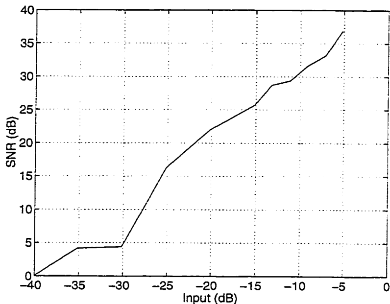
Figure 7.44: Dynamic range plot for NRZ modulator in 20MHz bandwidth.
